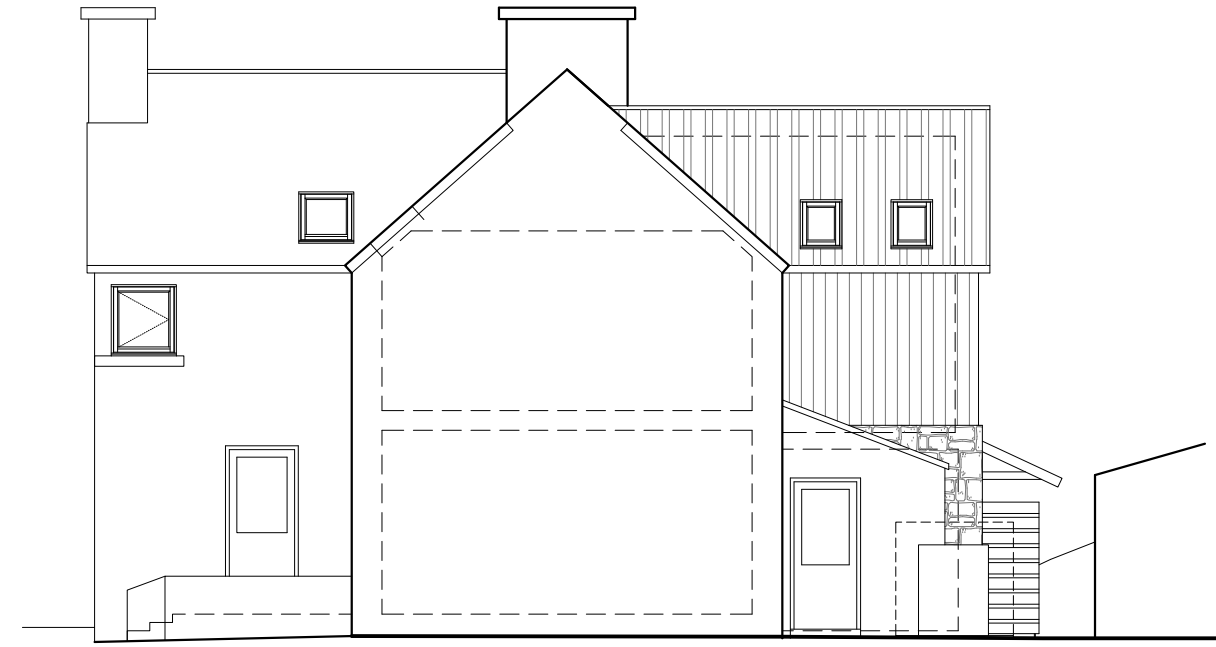
4 WEST ELEVATION as proposed
